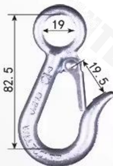
750LBS SPRING HOOK/0.34 TONS UNIT: MM/WEIGHT: 0.22KG
