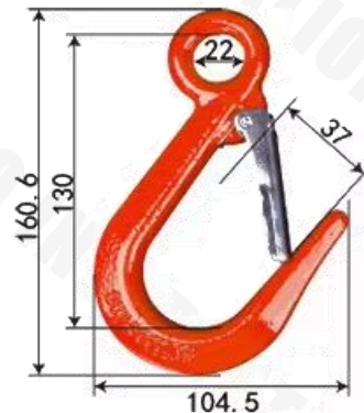
5000 LB WIDE MOUTH HOOK / 2.2 TONS UNIT: MM/WEIGHT: 0.44KG
