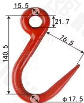
1T STEEL PIPE HOOK UNIT MM/WEIGHT 0.55KG
